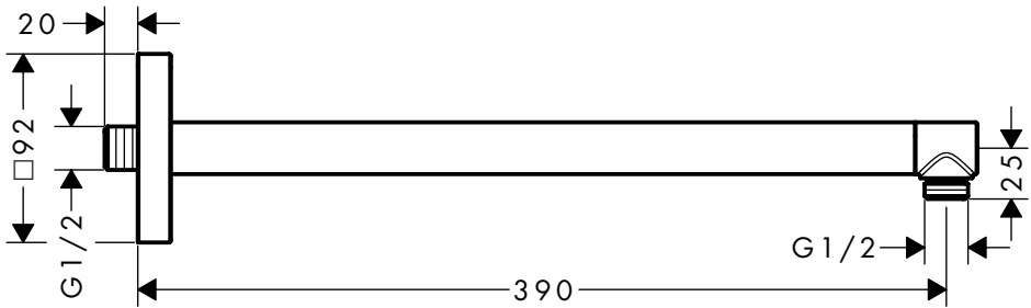
AXOR ShowerSolutions 390 mm softsquare 26967XX0 / 26967XX7
