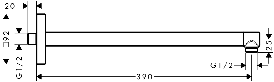
AXOR ShowerSolutions 390 mm square 26436XX0 / 26436XX7
