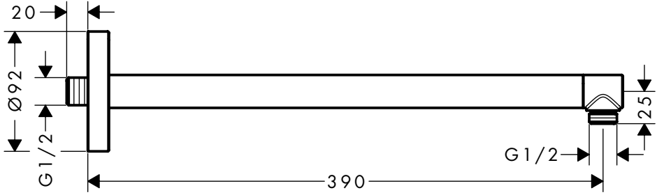
AXOR ShowerSolutions 390 mm round 26431XX0 / 26431XX7
